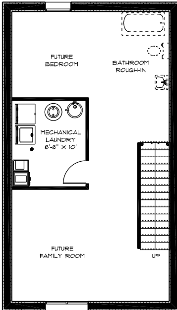
UNFINISHED BASEMENT 720 SQ/FT
