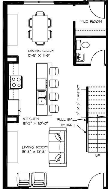
MAIN FLOOR 720 SQ/FT
